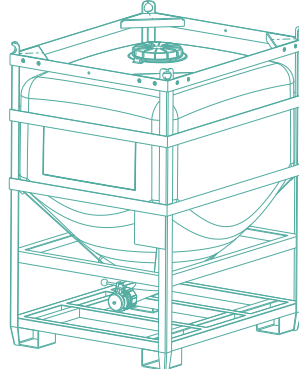
TS 5106: Front view
